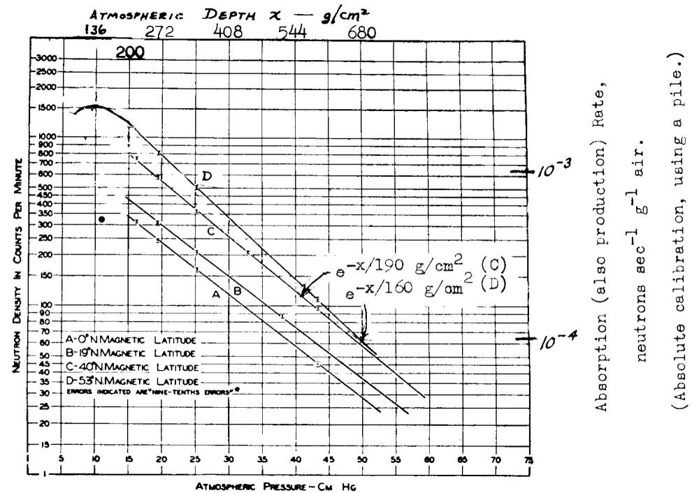
FIG. X.3 Apparent absorption of neutron-producing radiation at various magnetic latitudes*. See text, p. 220.
